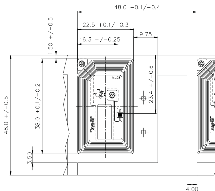
Figure 2-4. Dimensions of Tag-it HF-I Pro Transponder Inlay Rectangle – Miniature (RI-I03-114A-S1)
